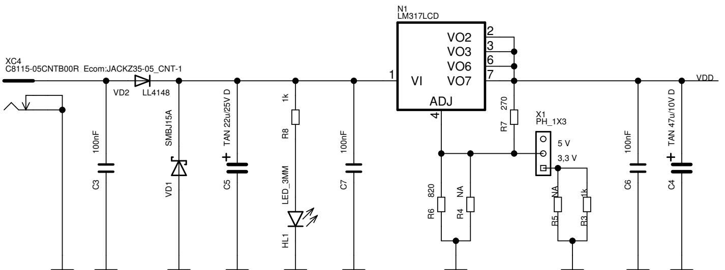
Resistor Set Oscillator, 1kHz to 33MHz Frequency Range BY OK1CJH 2016
